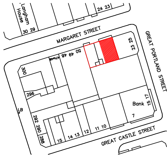
Location Plan - 1:1250
